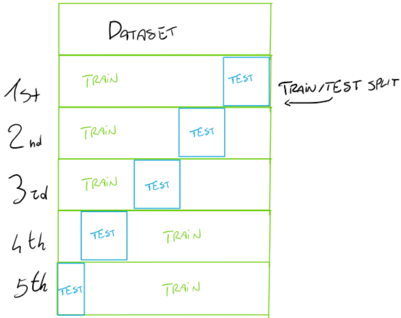
Figura 1.11 Cross-Validation.
